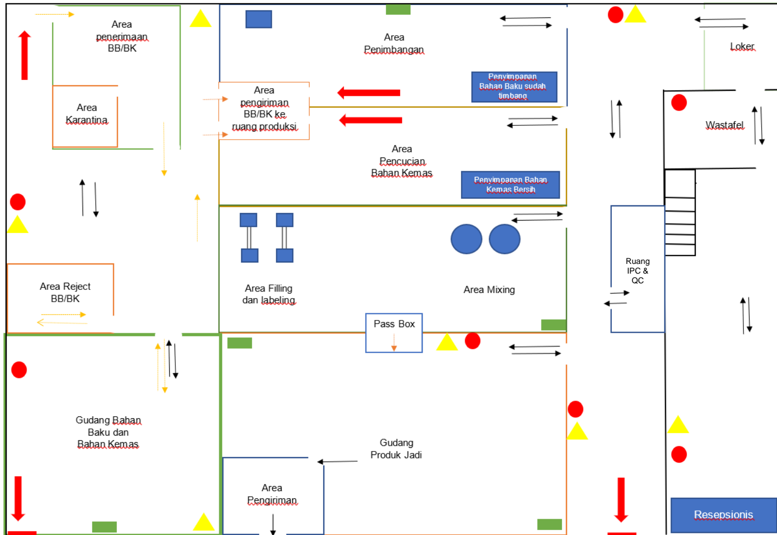
Denah Lantai 1
